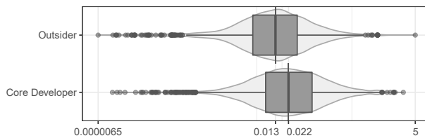
Fig. 6. Comparison of lambda ratio per lines of code added
